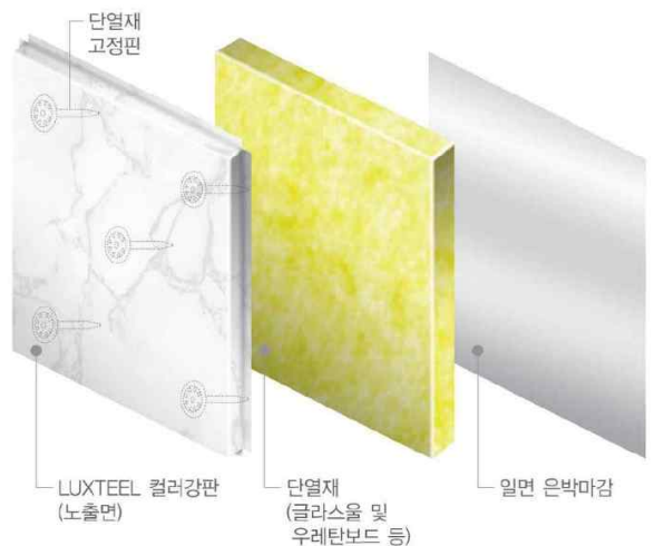
● 일면 BACK PANEL ●
